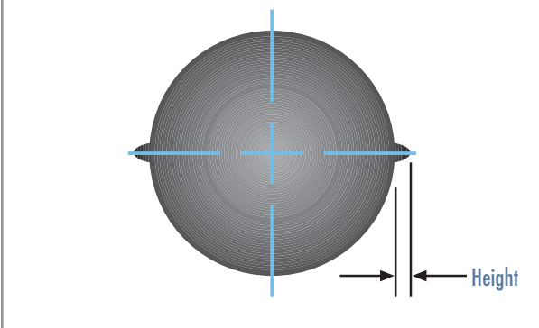
Parting line projection diagram
